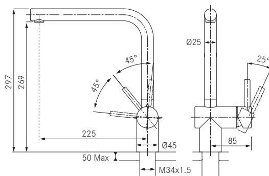
Tap Atlas Neo Nozzle side HP SS Version
